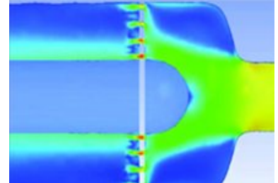
UV chamber design with special flow management system - optimised using CFD techniques.
